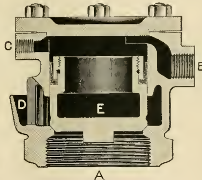
SECTION OF STAR AUTOMATIC CYLINDER RELIEF VALVE.
